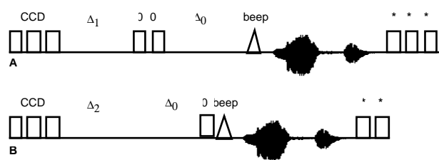
Fig. 3: Synchronization Protocols
